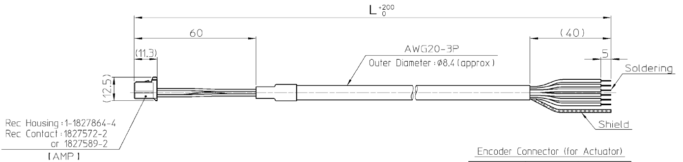
External view of extension cable for absolute encoder
