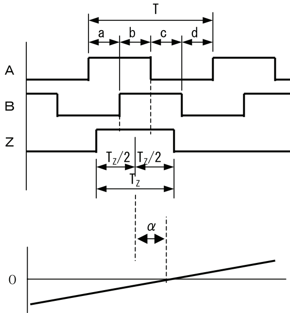
Fig. 1 A, B and Z signal and relationship with U-N motor EMF waveform with CW rotation facing the output flange end
