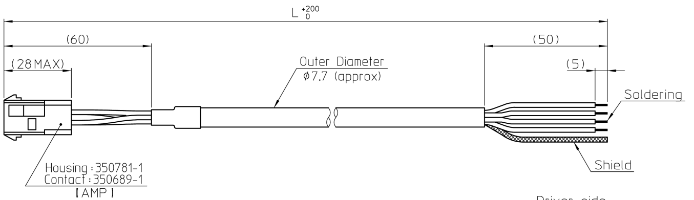
External view of extension cable for motor
