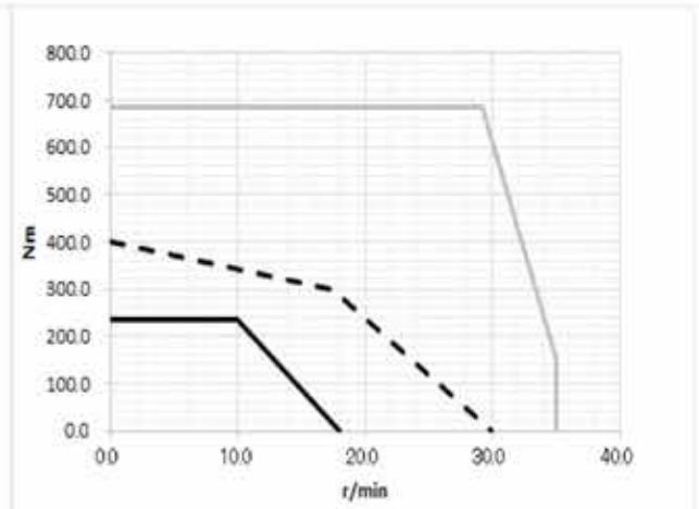
FHA-40C-100-H
