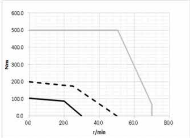
FHA-40C-50-H
