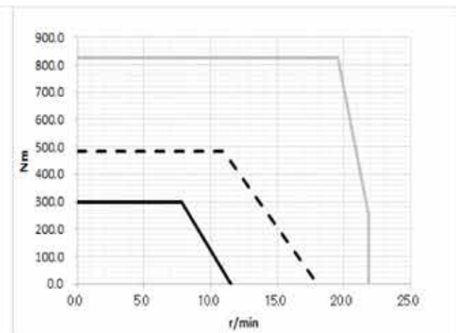
FHA-40C-160-H
