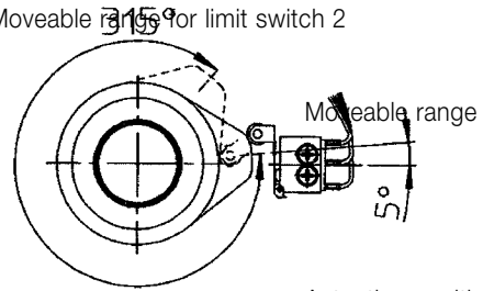
Actuating position
