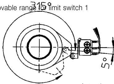
Actuating position
