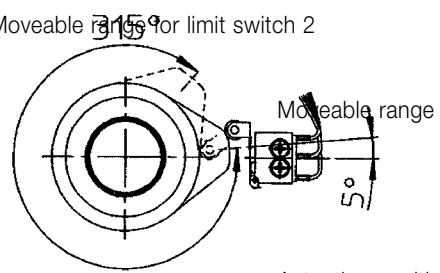
Actuating position
