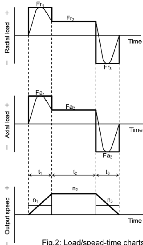
Fig.2: Load/speed-time charts
