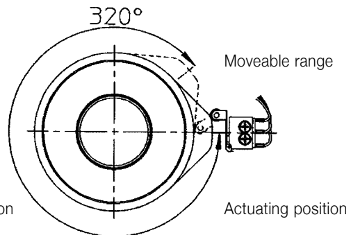
Movable range for limit switch 2
