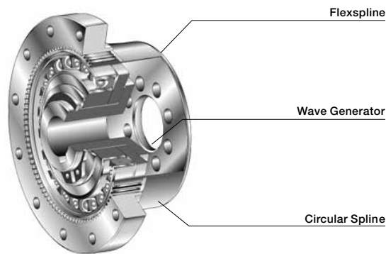
Structure of Harmonic Drive™ component product
