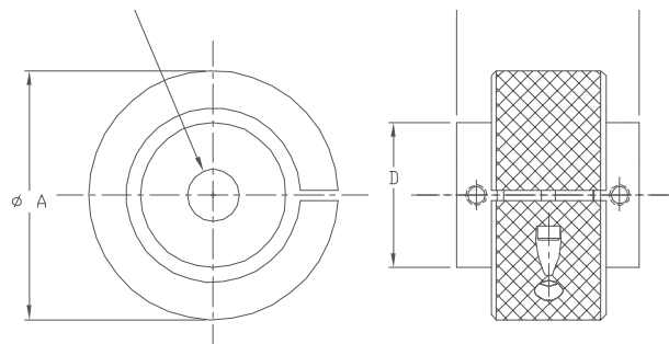
IN-LINE SHAFT
