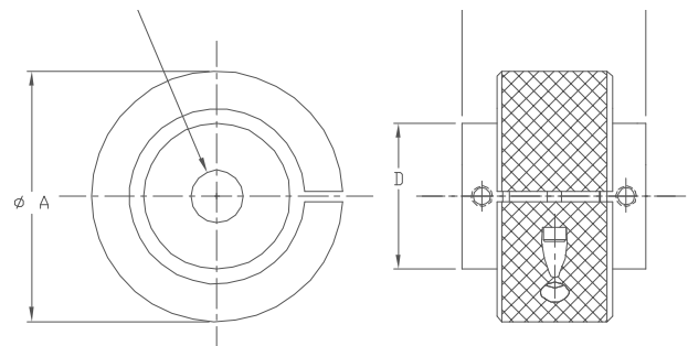
IN-LINE SHAFT
