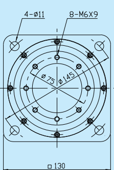
RFS-25-XX12-TE With Tach-Generator and Encoder
