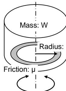
Example of rotary torque calculation (friction coefficient = 0.1) SHA: 20% torque of maximum torque is shown.
