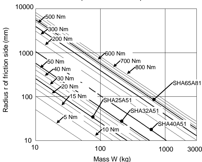
Example of rotary torque calculation (friction coefficient = 0.1) SHA: 20% torque of maximum torque is shown.
