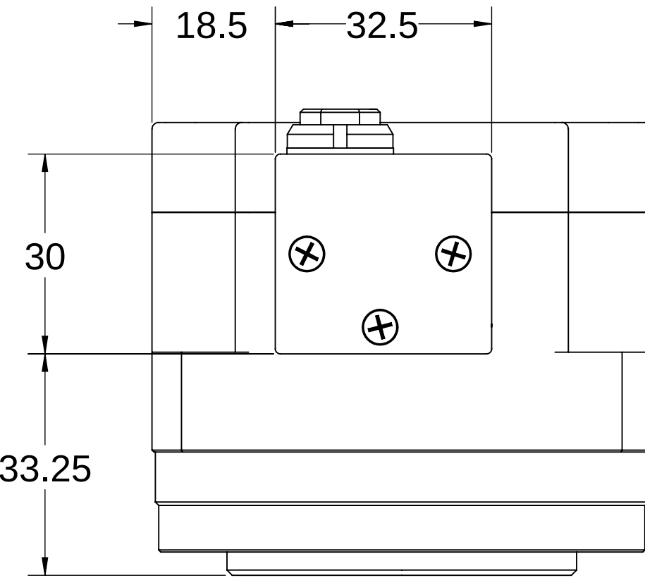
PM1 OPTION REAR EXIT
