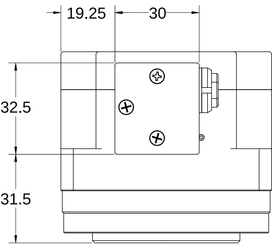
PM2 OPTION RIGHT EXIT
