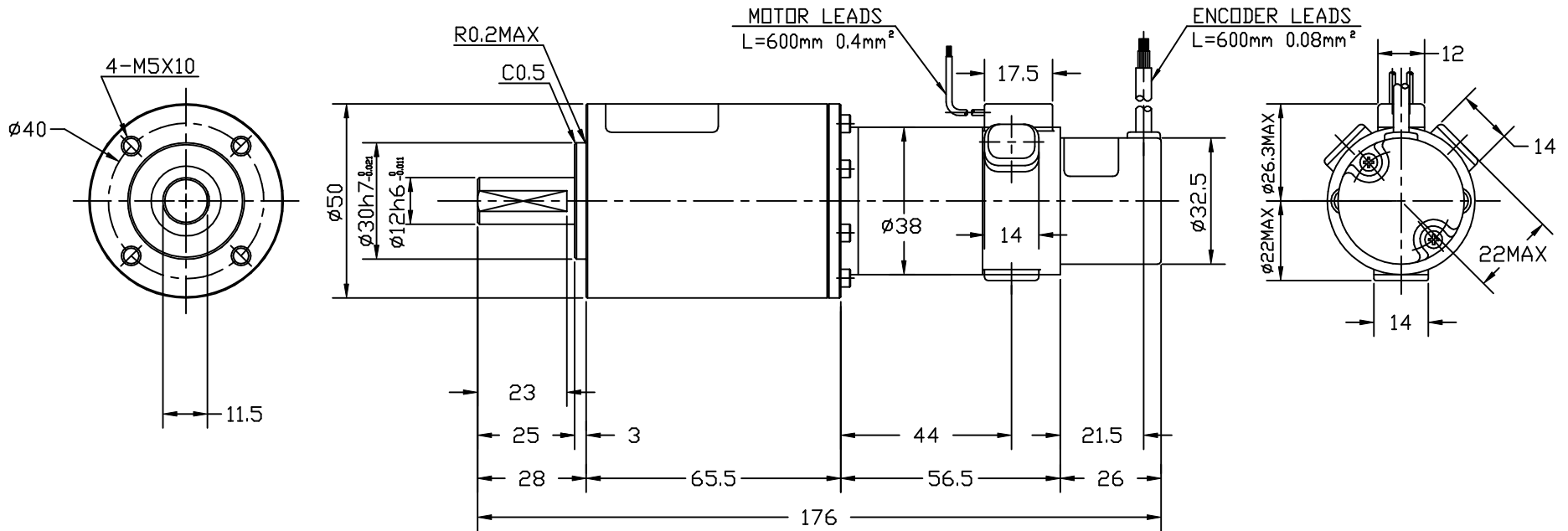
RH-14D-XX02-E100XX actuator with incremental encoder
