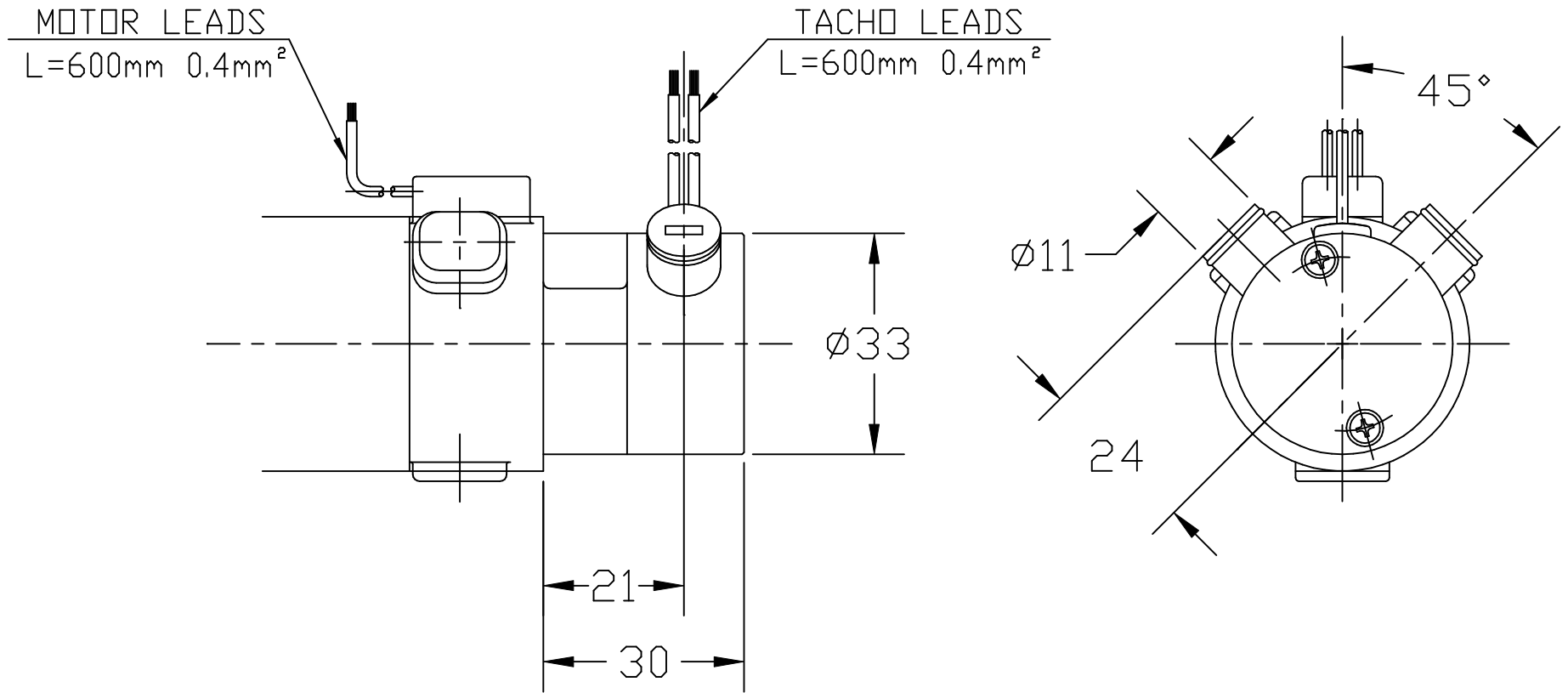
RH-8D,11D,14D Tacho Generator Version
