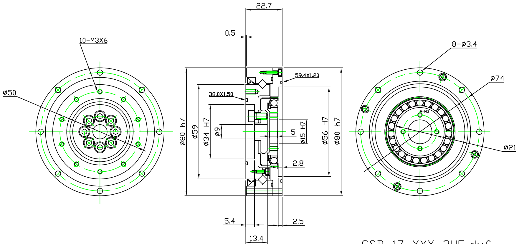
CSD-17-XXX-2UF,dxf
