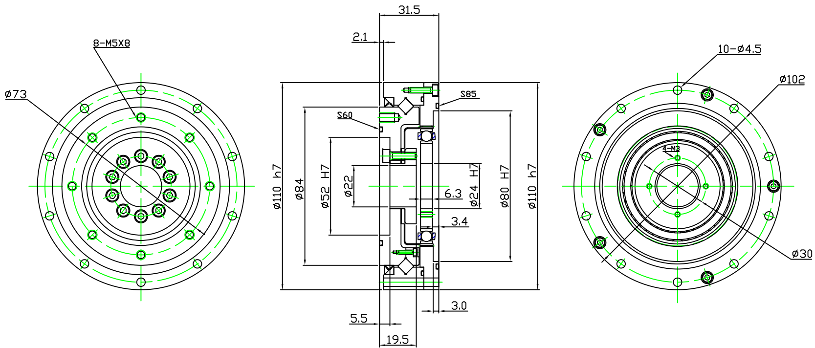
CSD-25-XXX-2UF.dxf
