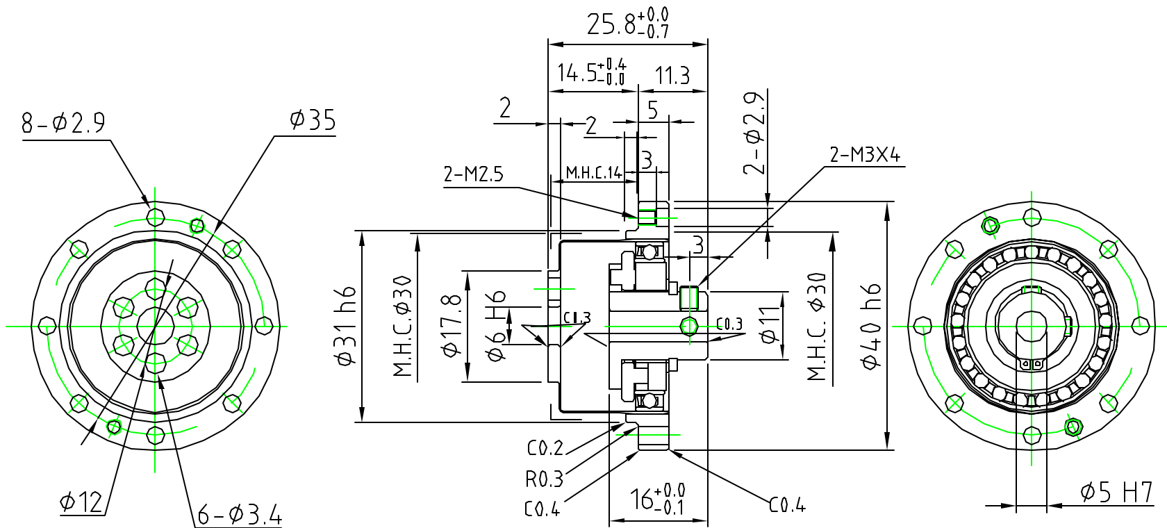
CSF-11-XXX-2A-R.dxf
