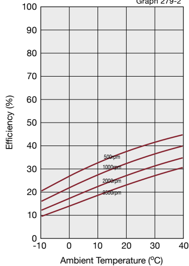
Ratio 50 Size 17, 20, 25, 32, 40
