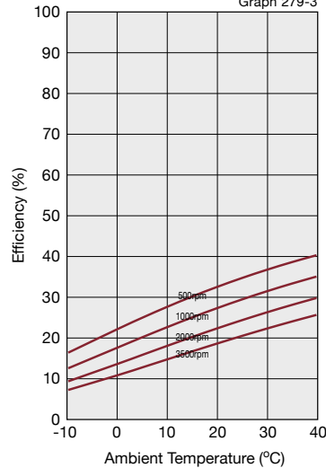
Ratio 80, 100, 120 Size 17, 20, 25, 32, 40
