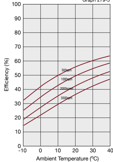
Graph 279-5
