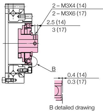
Size 14,17 Configuration of wave generator
