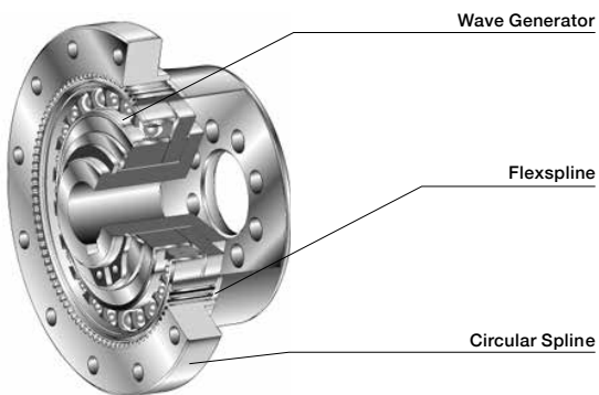
Structure of Harmonic Drive® component product
