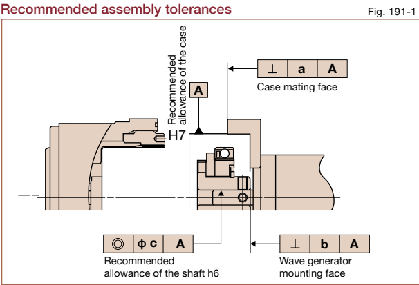
Recommended assembly tolerances
