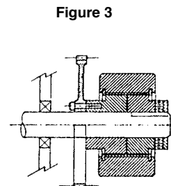
Concentric Shaft
