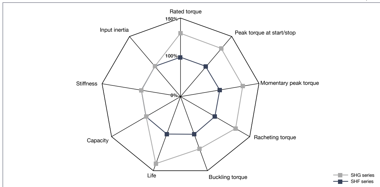
Comparison between SHG series and SHF series
