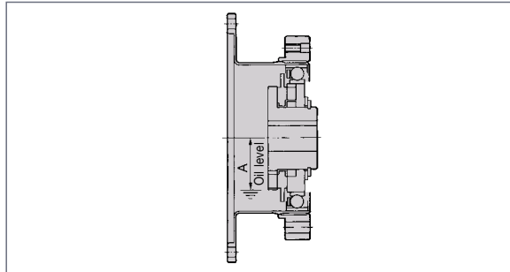
Oil level for horizontal use
