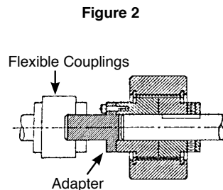
In-Line Shaft
