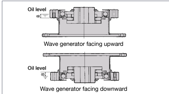
Oil level for vertical use
