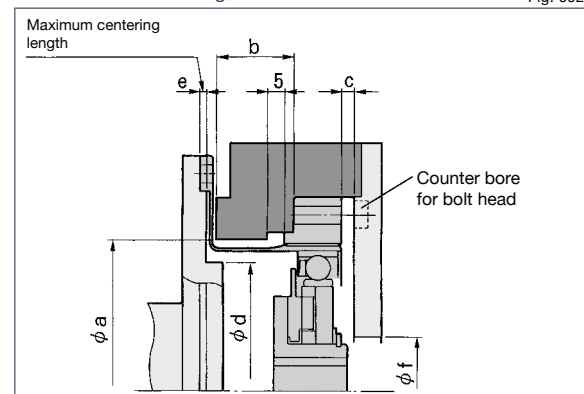
Recommended housing dimensions
