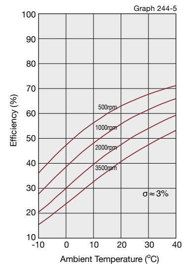
SHG/SHF-14 to 65 Ratio 160
